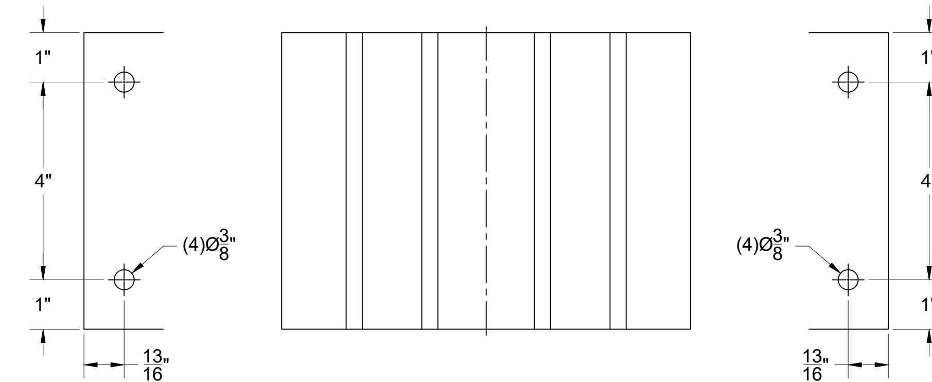
FMB51_ 135° INSIDE FASCIA MOUNT BRACKET
