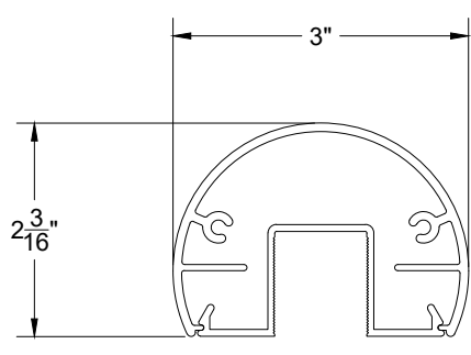
X3T20 SIERRA SERIES TOP RAIL
