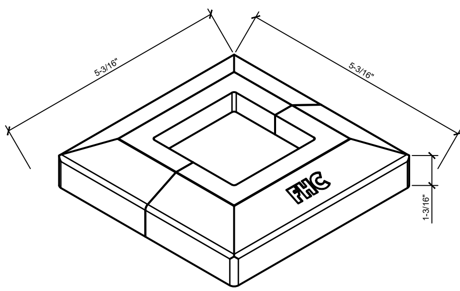
CV2 - COVERS FOR 2-3/8" SQUARE POSTS
