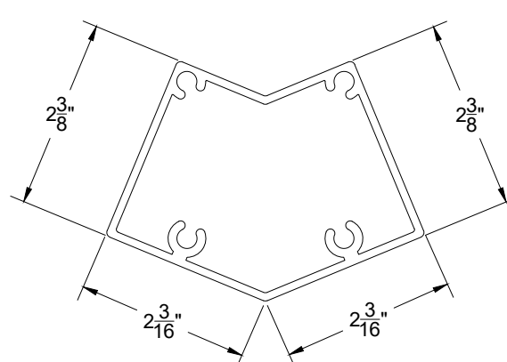
SP520 135 DEGREE POST
