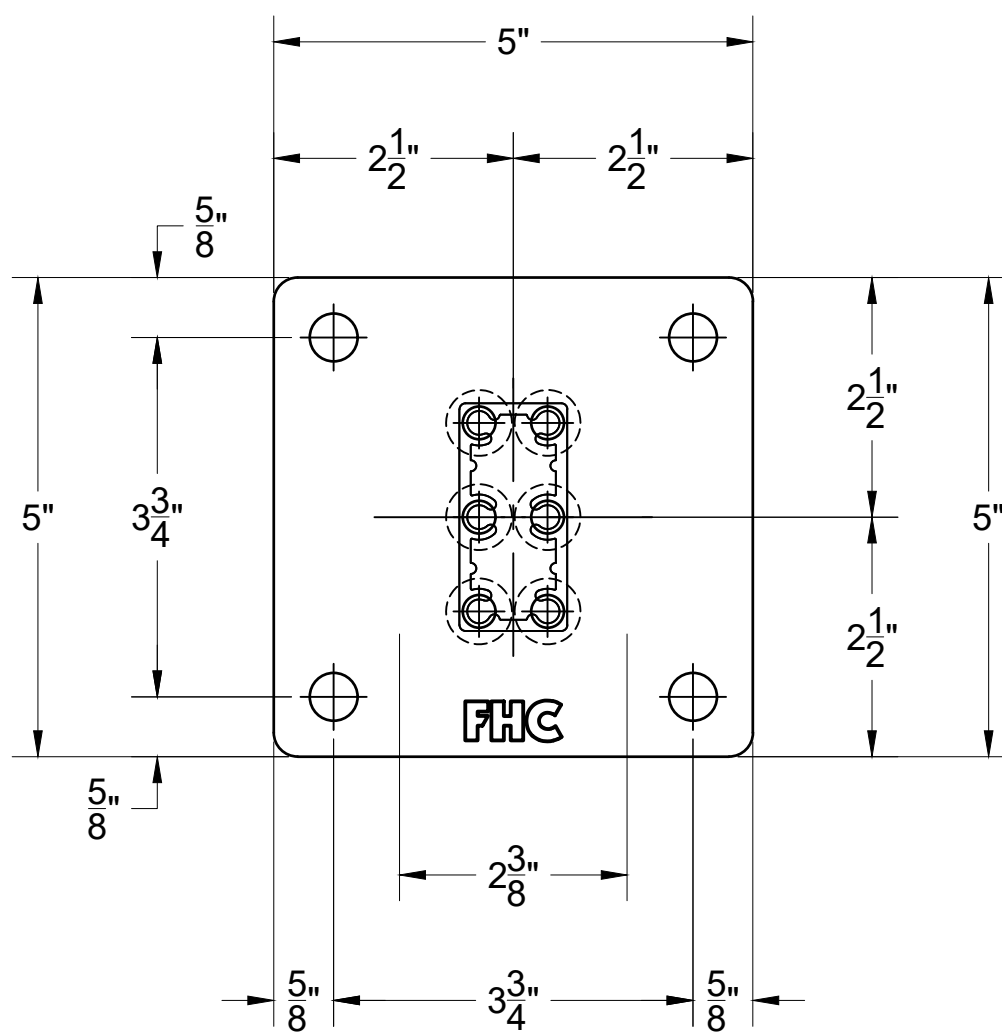
SBP2 - RECTANGULAR POST BASE PLATE
