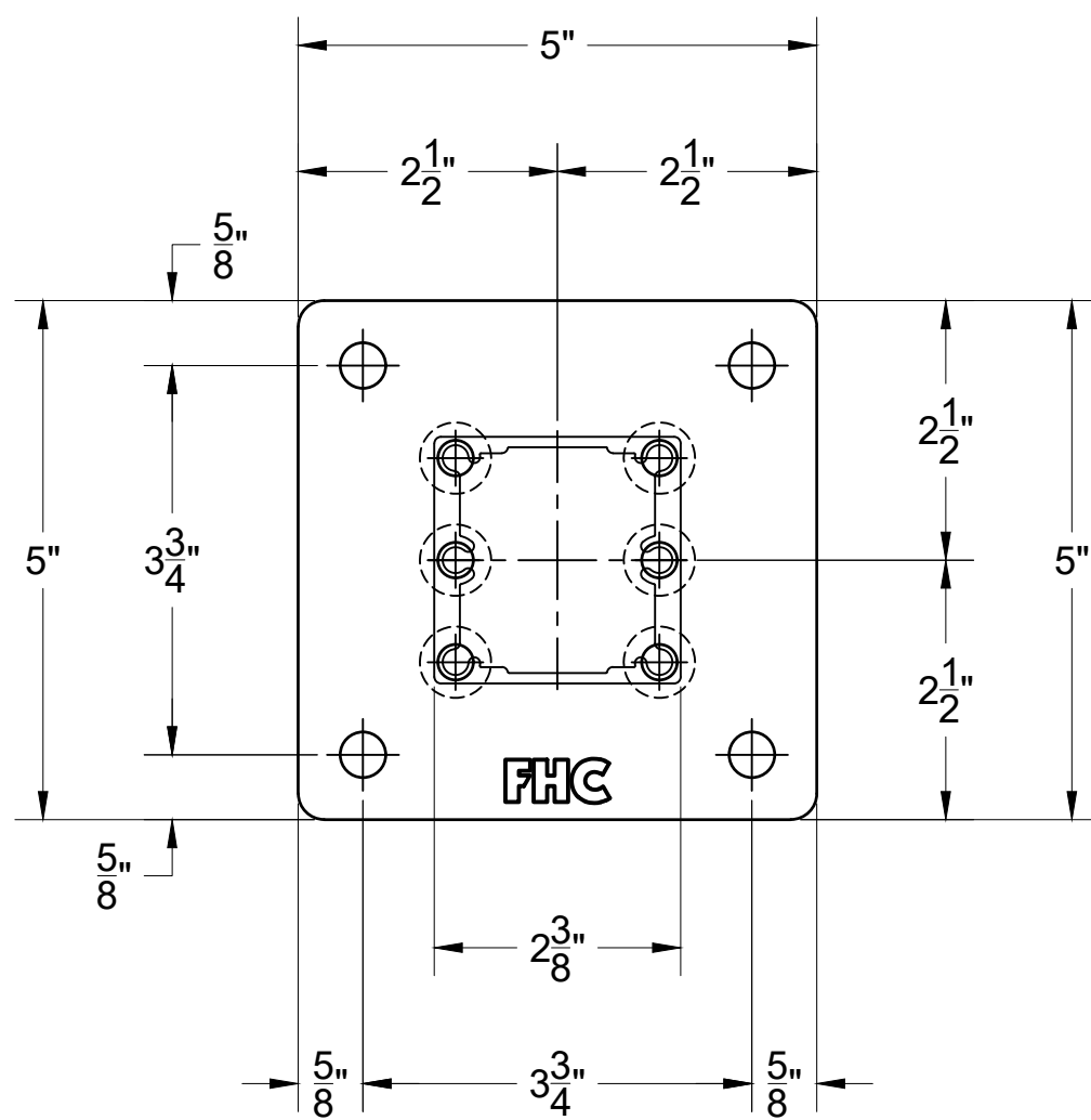
SBP5 - STANDARD POST BASE PLATE
