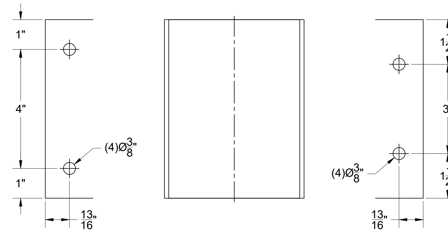
FMB5_ 135° OUTSIDE FASCIA MOUNT BRACKET
