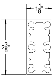
SL20 2-3/8" X 1-1/8" SLIM POST
