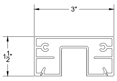
X2T20 TAHOE SERIES TOP RAIL
