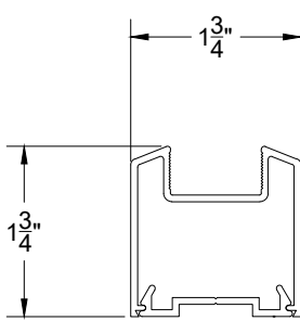
BRG20 AR BOTTOM RAIL FOR GLASS INFILL
