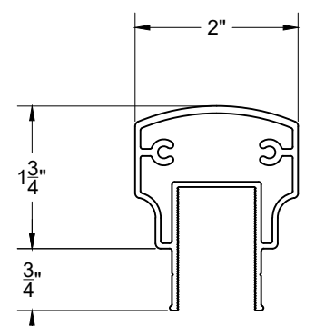
X1T20 ARROWHEAD SERIES TOP RAIL
