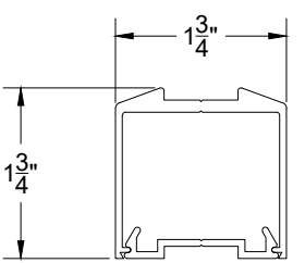
BRP20 AR BOTTOM RAIL FOR GLASS INFILL
