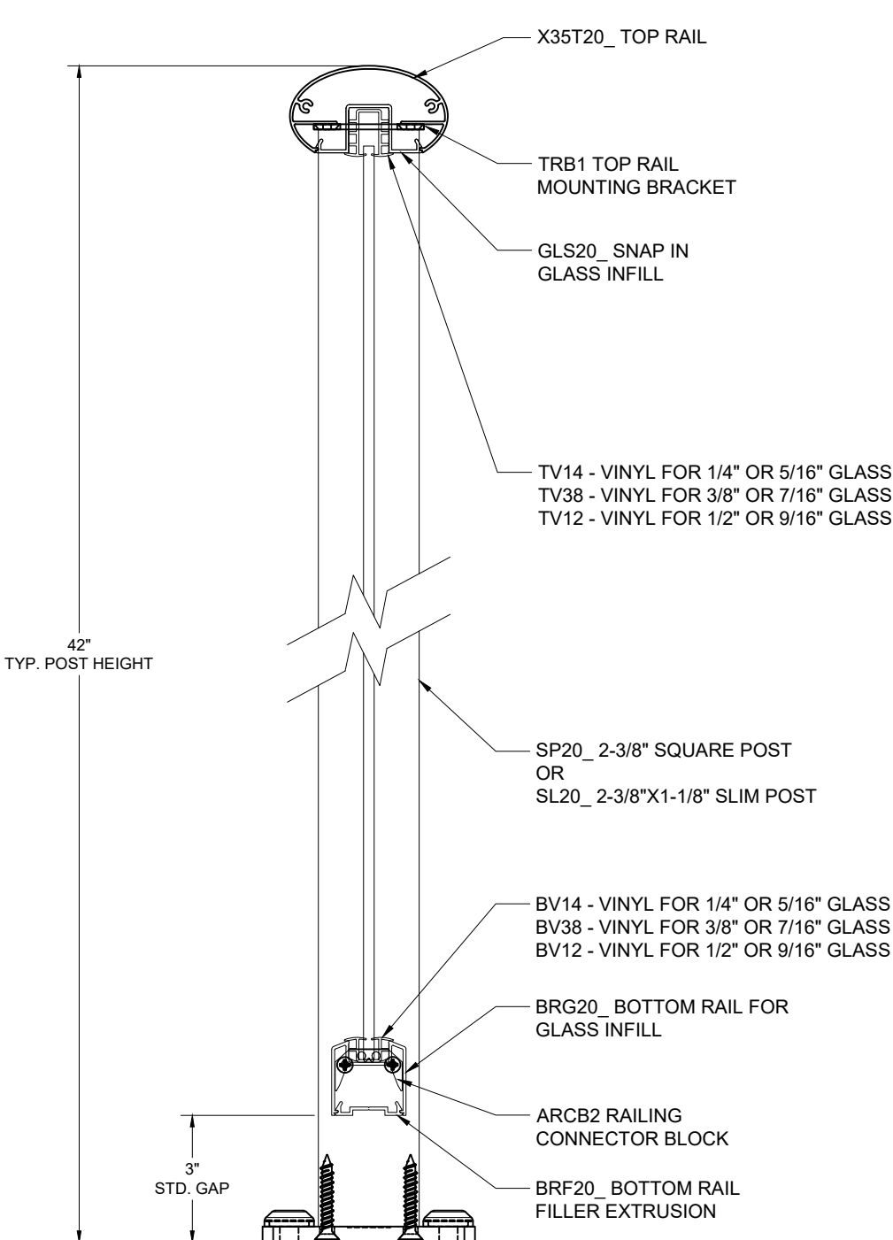
X2 TAHOE SERIES RAILING TYPICAL SECTION VIEW
