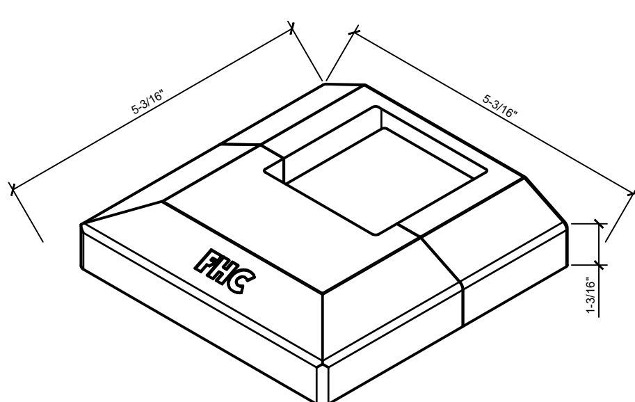
CV02 - OFFSET COVERS 2-3/8" SQUARE POSTS
