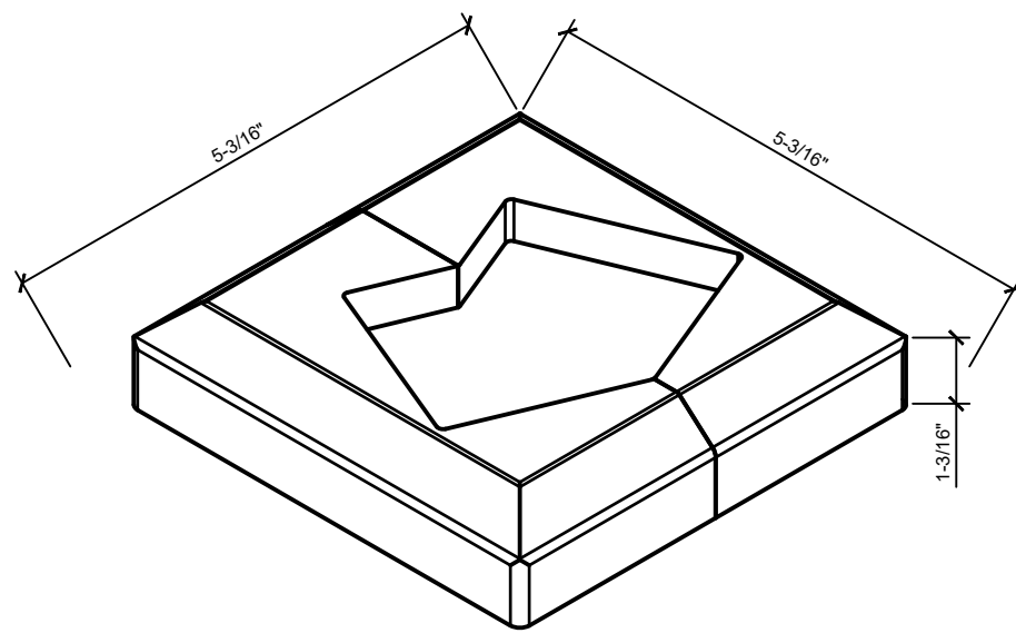
CV135 - COVERS 135° SQUARE POSTS
