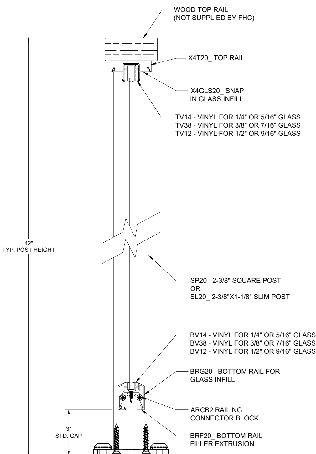
X2 TAHOE SERIES RAILING TYPICAL SECTION VIEW
