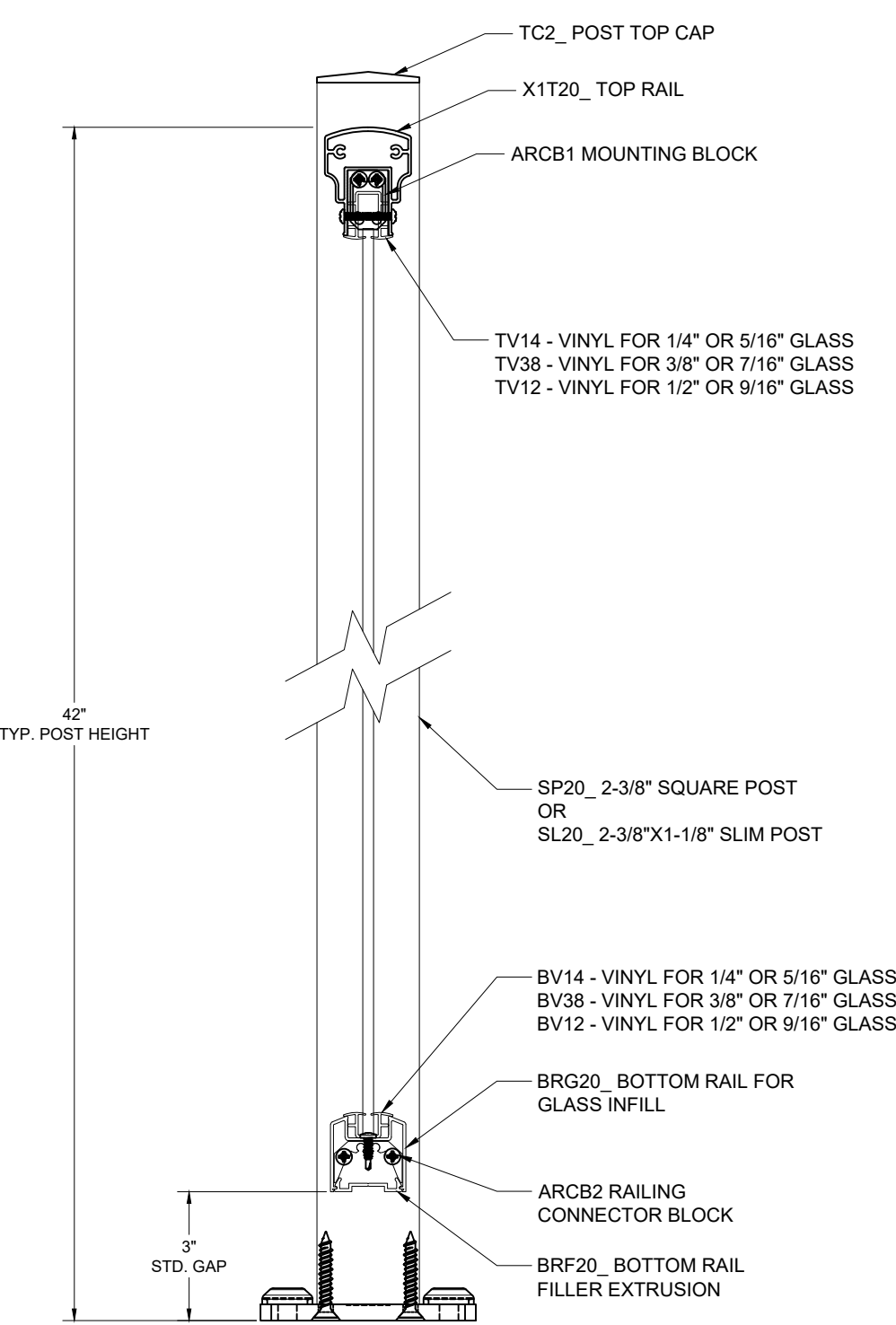
X1 ARROWHEAD SERIES RAILING TYPICAL SECTION VIEW
