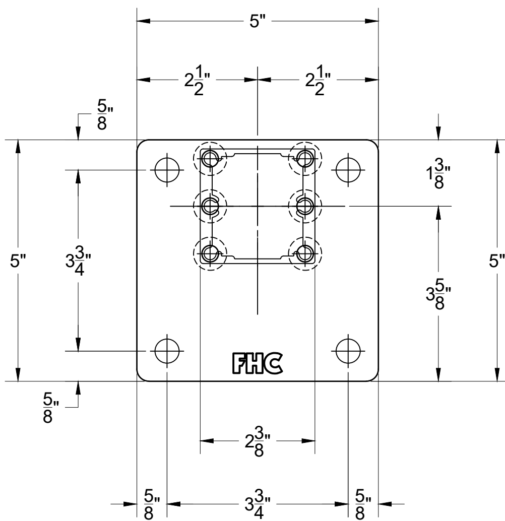
0BP5 - OFFSET STANDARD POST BASE PLATE
