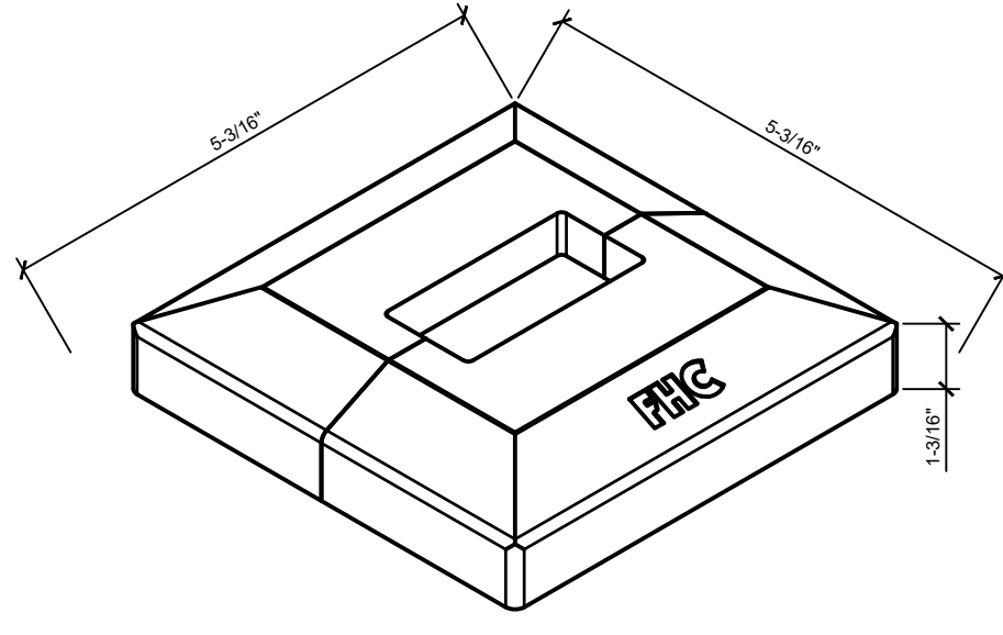
CV1 - COVERS FOR 1-1/8" X 2-3/8" SLIM POSTS
