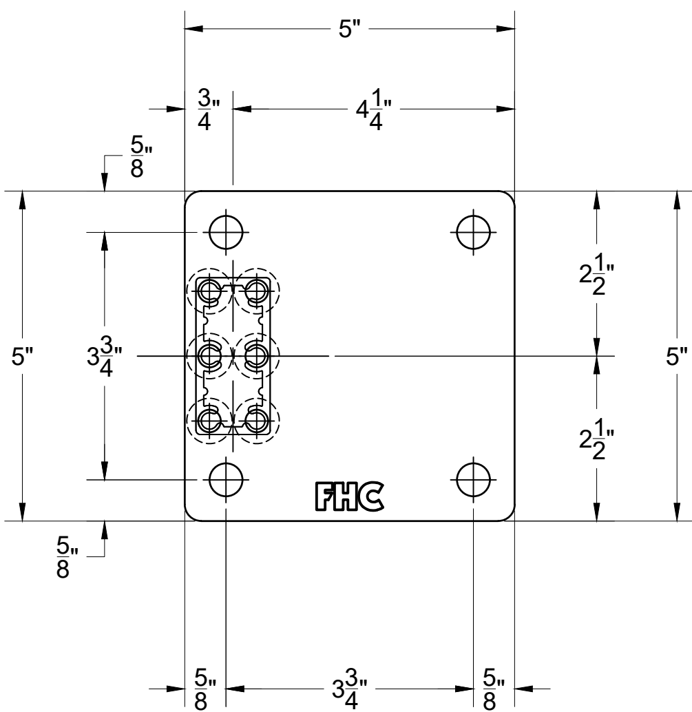
0BP2 - RECTANGULAR POST BASE PLATE
