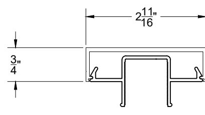
X4 FUJI SERIES TOP RAIL
