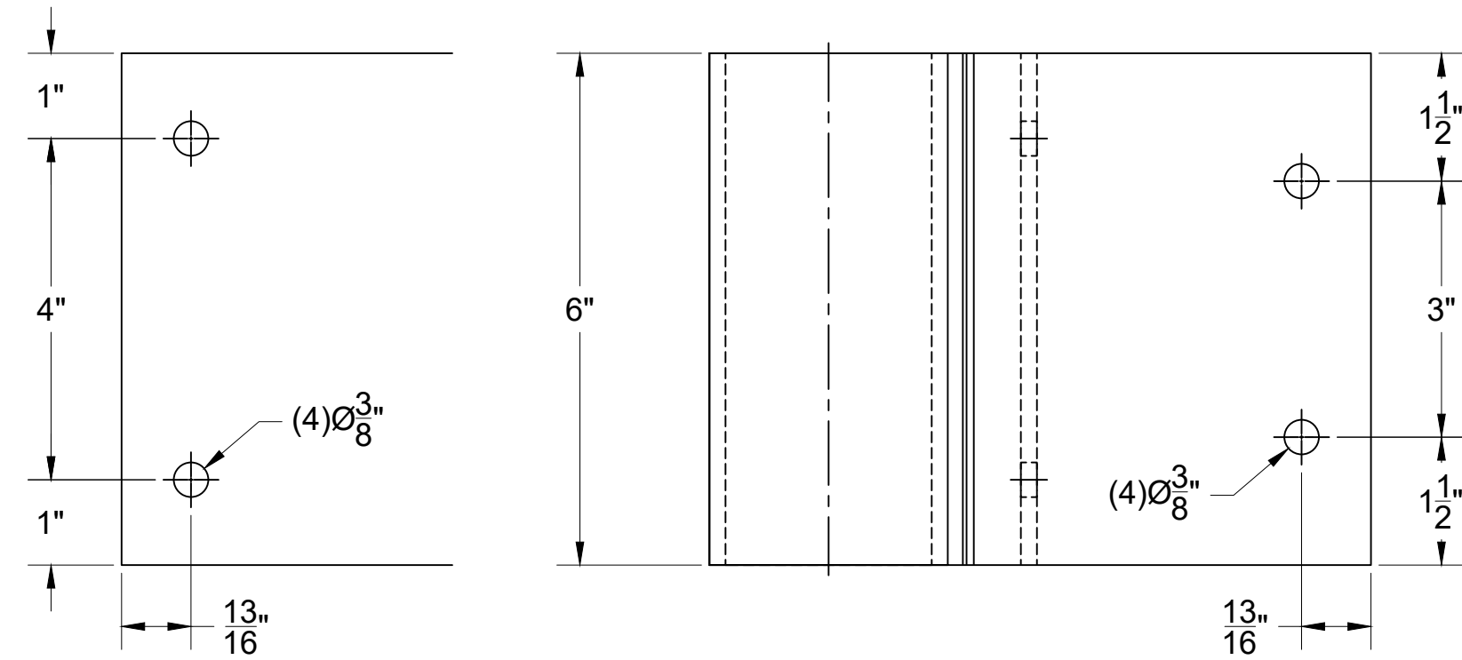
FMB90_ 90° OUTSIDE FASCIA MOUNT BRACKET
