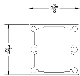
SP20 2-3/8" SQUARE POST
