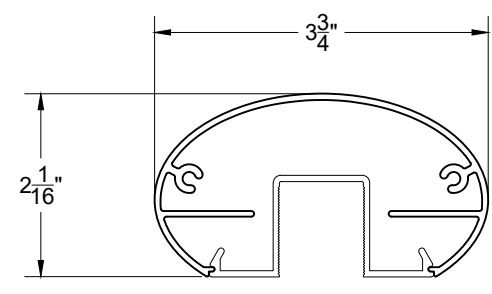
X35 EVEREST SERIES TOP RAIL
