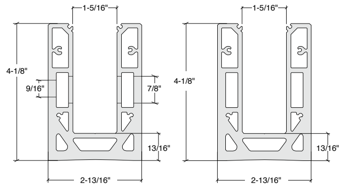
F Profile Fascia/Side Drilled and Counterbored 12" On Center and 6" From Each End
