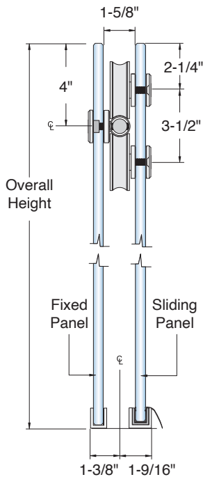
Section View of Sliding Shower Kit
