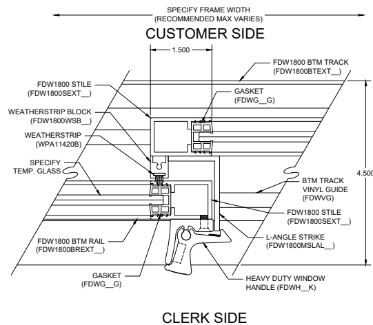
D8 MEETING STILE DETAIL
