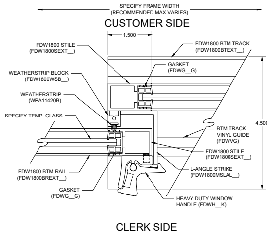
D7 MEETING STILE DETAIL
