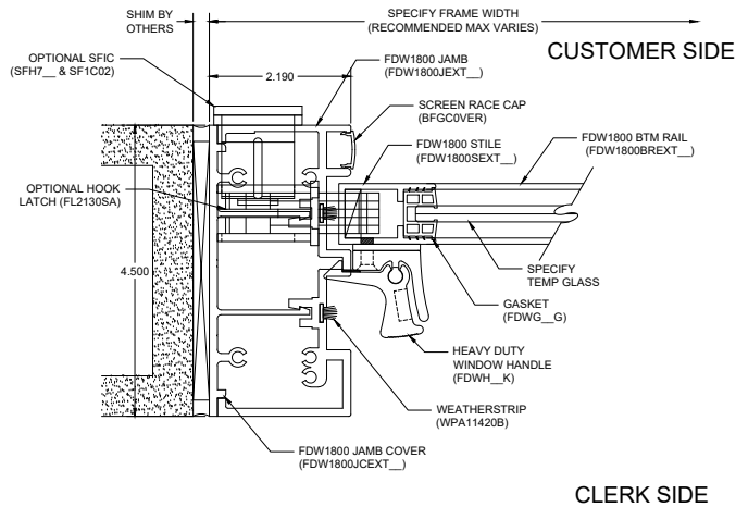
C3 JAMB & WALL DETAIL
