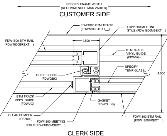
D4 MEETING STILE DETAIL
