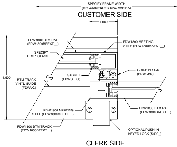
D5 MEETING STILE DETAIL
