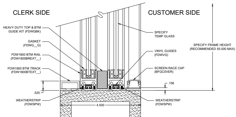
B3 SILL DETAIL FDW4200 DELUXE SERVICE WINDOW SCALE: FULL
