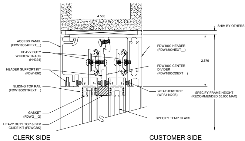
A3 HEADER DETAIL (MANUAL CLOSING) FDW4200 DELUXE SERVICE WINDOW SCALE: FULL
