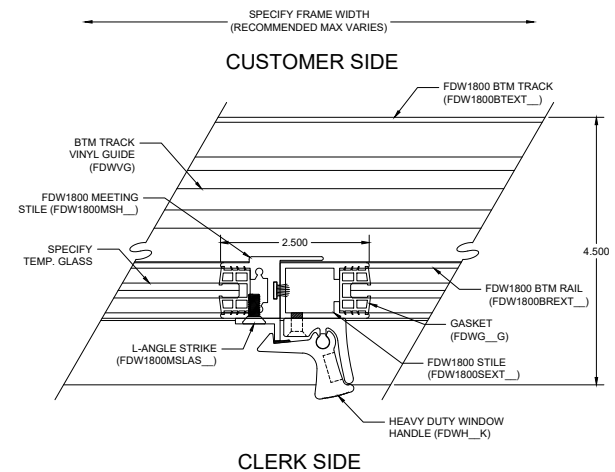
D10 MEETING STILE DETAIL
