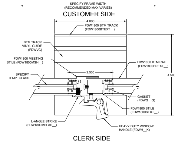
D9 MEETING STILE DETAIL
