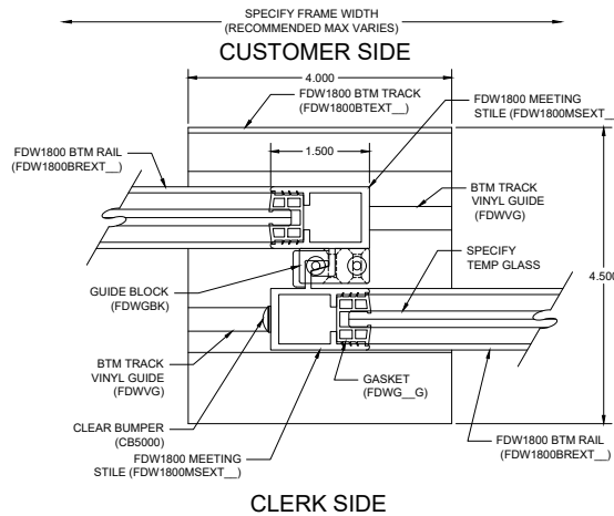
D3 MEETING STILE DETAIL
