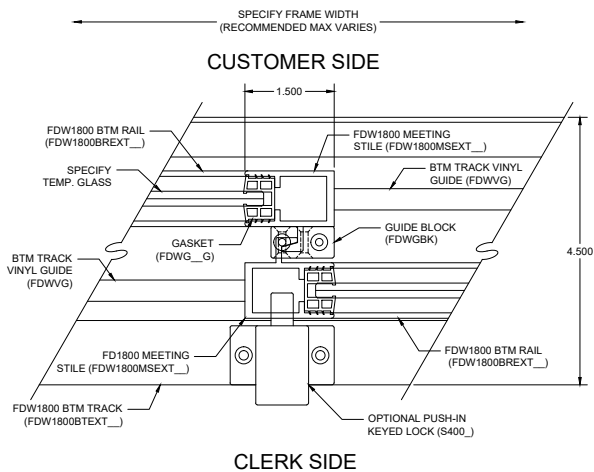
D6 MEETING STILE DETAIL
