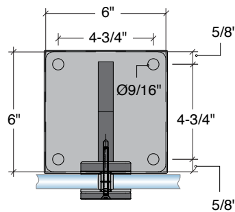
Center Post 3/8" Thick Base Plate With Cover
