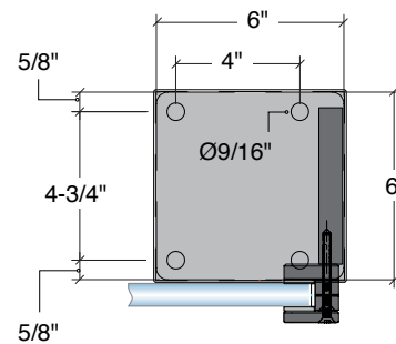
Right End 3/8" Thick Base Plate With Cover
