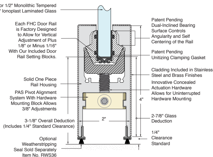
Square Profile End View Shown
