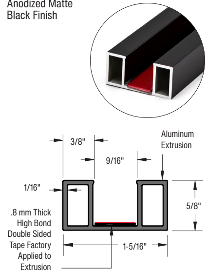
FHC Premium Perimeter Grid Channel For 1/2" Glass
