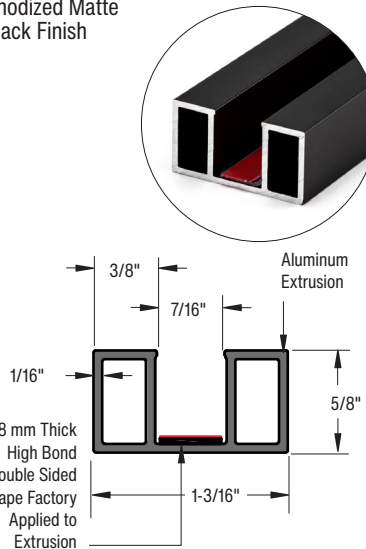
FHC Premium Perimeter Grid Channel For 3/8" Glass
