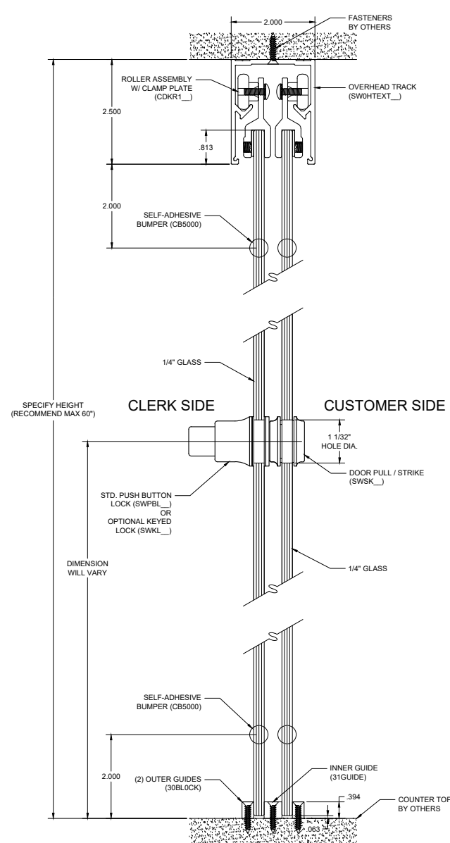
B HEADER & SILL DETAIL
