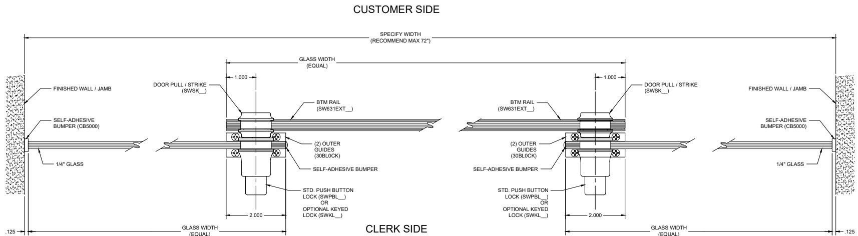
F WALL & MEETING DETAIL SHANNON PASS-THRU WINDOW
