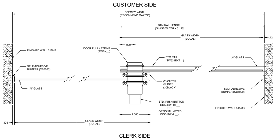
C WALL & MEETING DETAIL SHANNON PASS-THRU WINDOW
