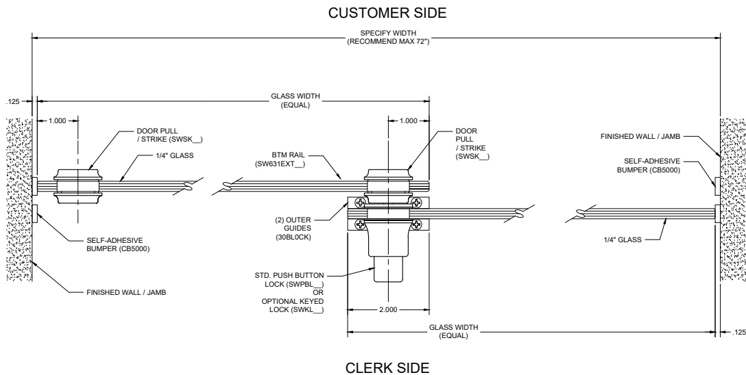
E WALL & MEETING DETAIL SHANNON PASS-THRU WINDOW
