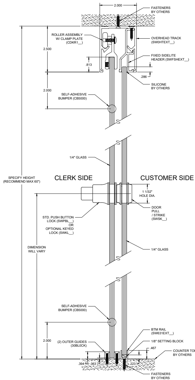
A HEADER & SILL DETAIL
