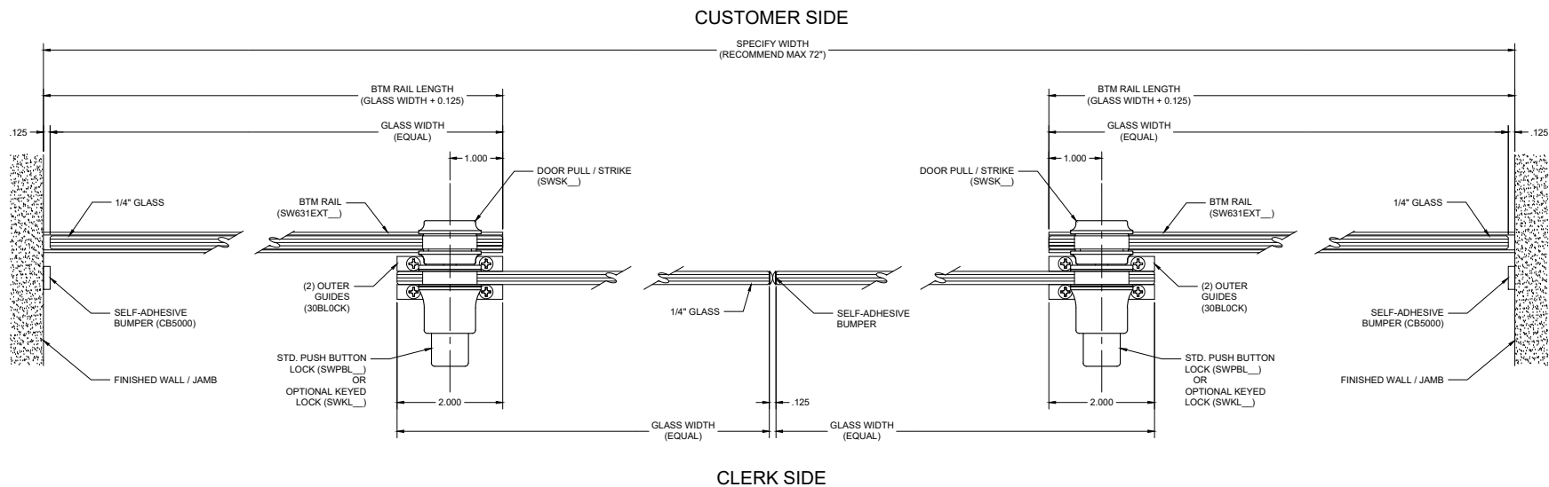
© WALL & MEETING DETAIL SHANNON PASS-THRU WINDOW
