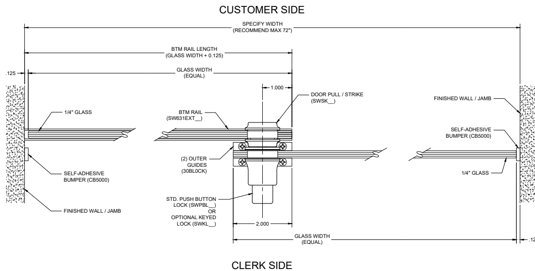
D WALL & MEETING DETAIL SHANNON PASS-THRU WINDOW
