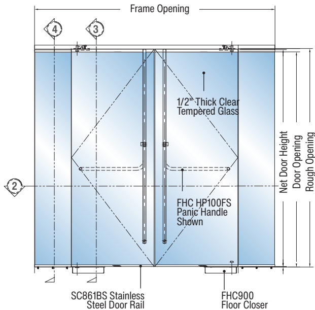
1 EXTERIOR ELEVATION VIEW
