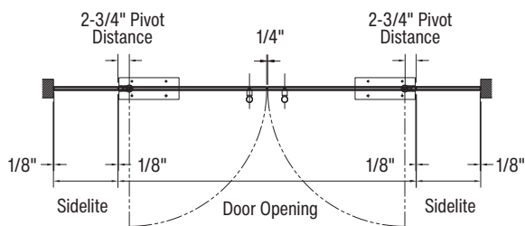
2 PLAN VIEW
