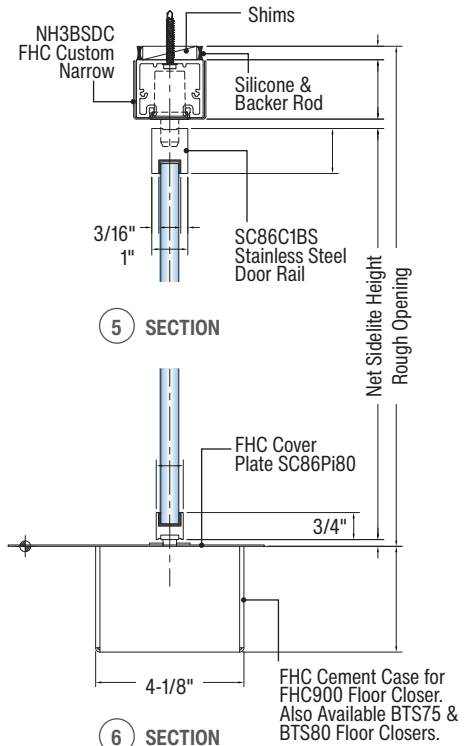
6 SECTION
