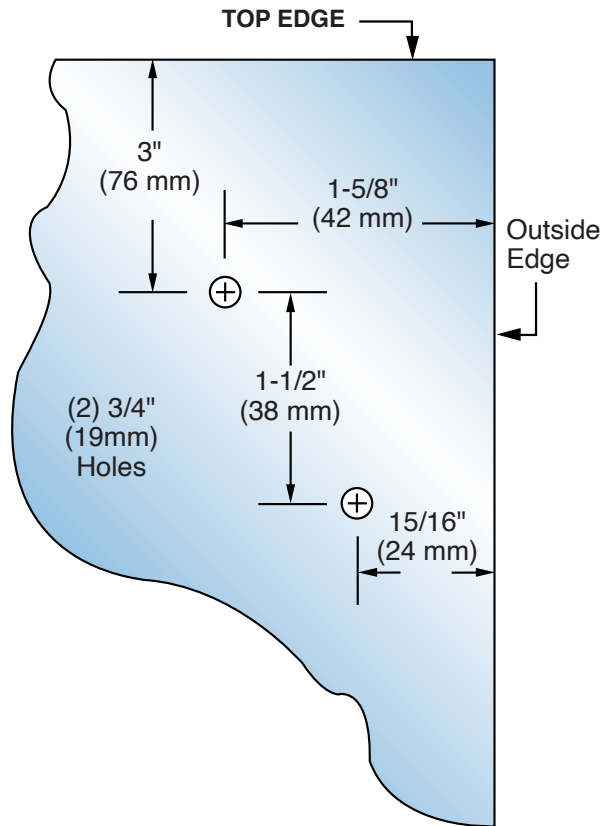
NAP90L (Left Side Return When Viewed From Outside)
