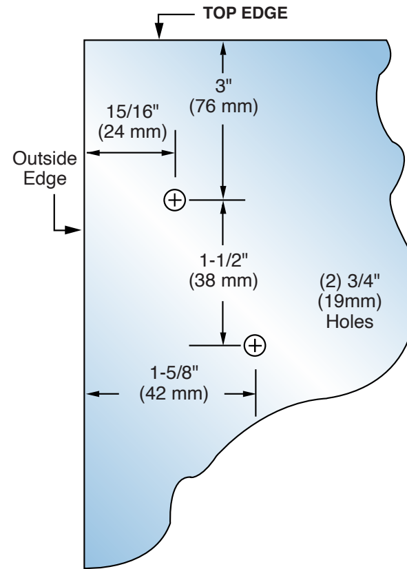
NAP90R (Right Side Return When Viewed From Outside)
