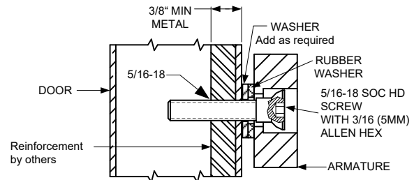
FIG. 2C REINFORCED DOOR
