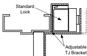
FIG. 1D Top Jamb Installation
